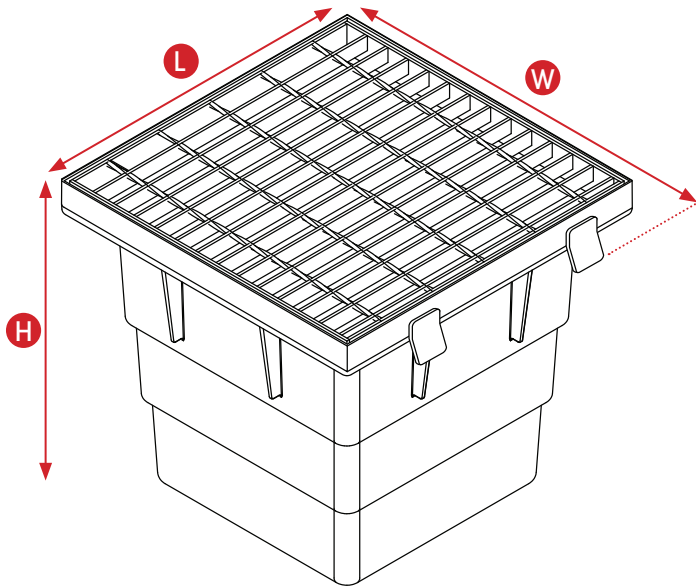
External Dimensions
